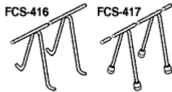
Continuous High Chair
